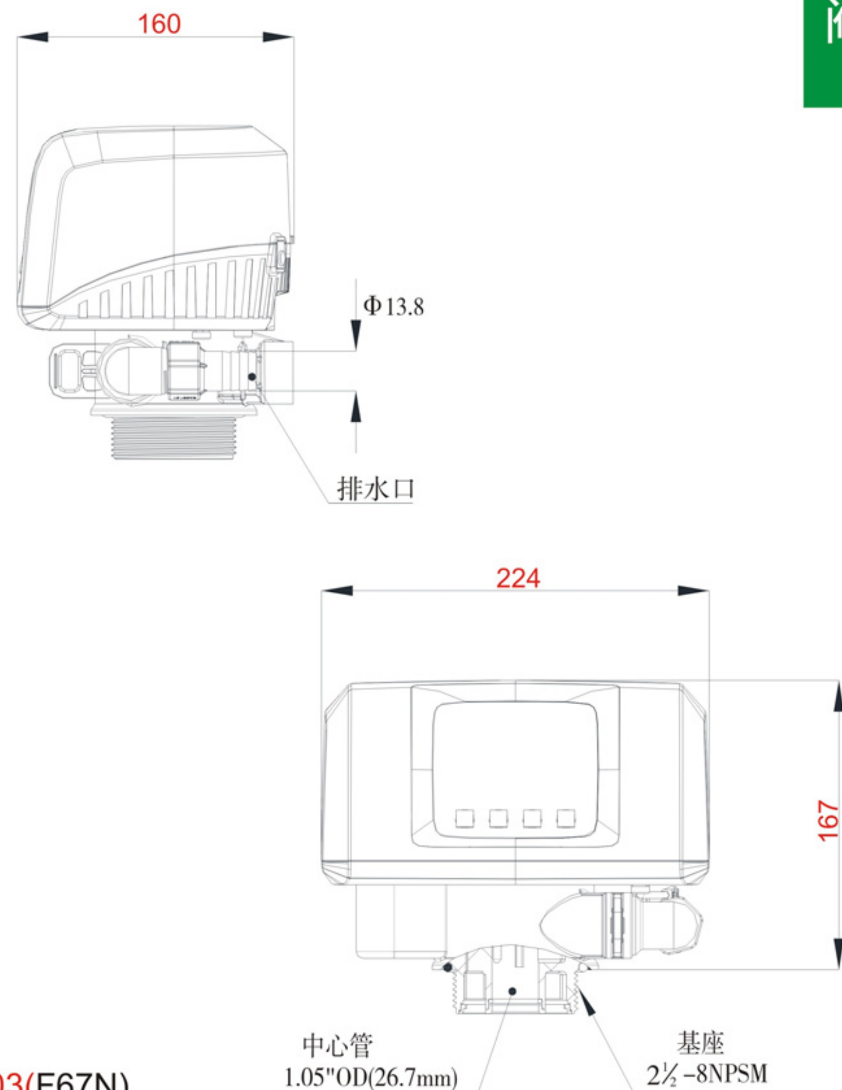
56603(F67N) 224 × 160 × 167mm
