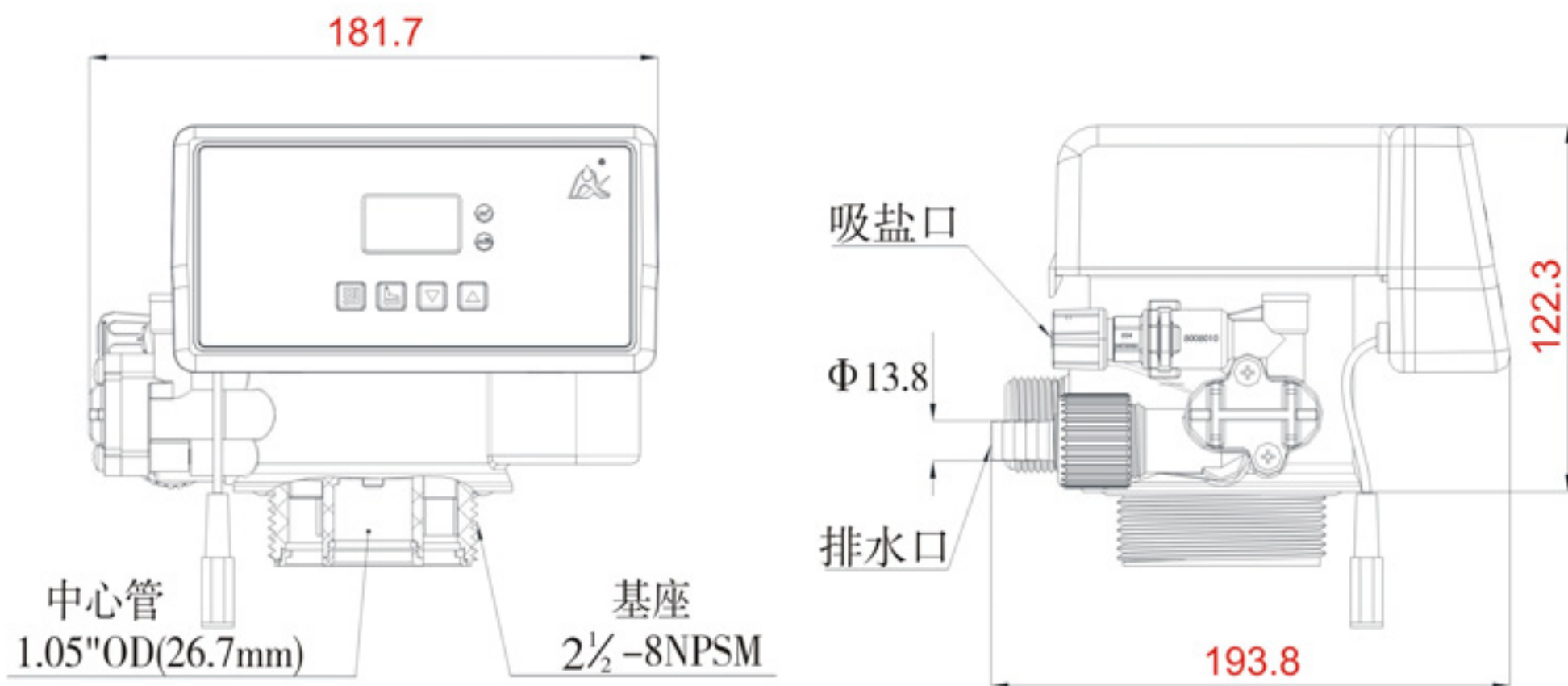
65603(F117Q3) 193.8 × 181.7 × 122.3mm
