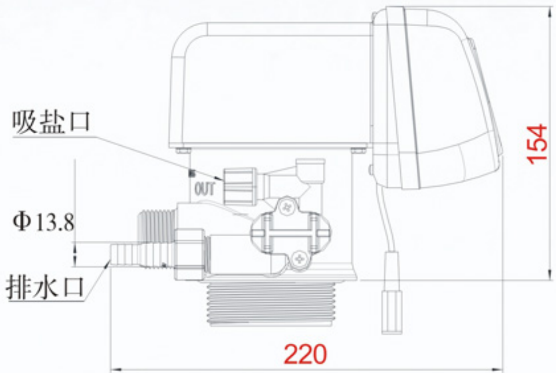
64604(F63P3) 220 × 182 × 154mm
