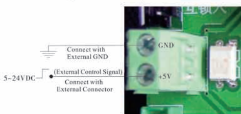
Figure13 Wiring of Remote Input
