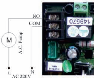
Figure10 Wiring of Booster Pump on Inlet Figure11 Wiring of Booster Pump on Inlet
