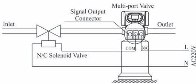
Figure 12 Wiring of Solenoid Valve on Inlet
