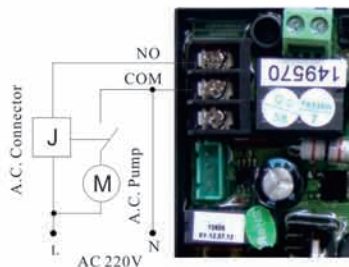
Figure10 Wiring of Booster Pump on Inlet Figure11 Wiring of Booster Pump on Inlet
