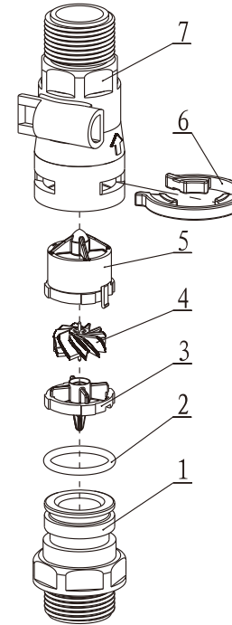
5447020 Flow Meter
