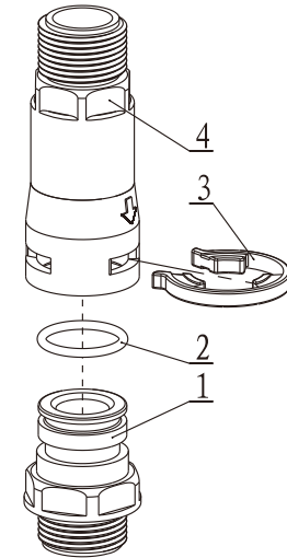
5457003 Animated Connector
