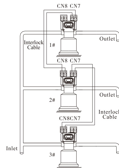
Figure 3-12 Interlock system
