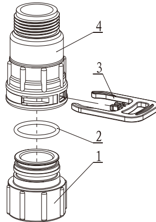
5457002 Animated Connector
