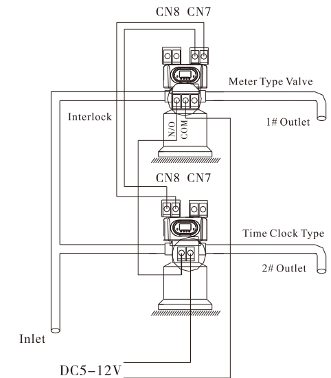
Figure 3-13 Series system
