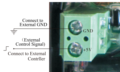
Figure 3-10 Wiring of Remote Handling Connector
