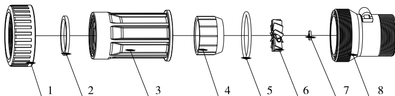
5447003 Flow Meter Components:
