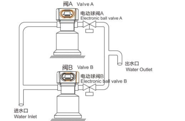
流量型控制阀+直通球阀+F91B控制阀一用一备软水系统 A one in service one standby softener system formed by flow meter type control valve+straight-way ball valve+F91B control valve
