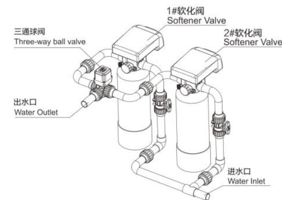
流量型控制+三通球阀一用一备软水系统 A one in service one standby softener system formed by flow meter type control valve+three-way ball valve
