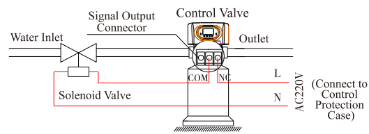
Figure 3-2 Wiring of Solenoid Valve on Inlet
