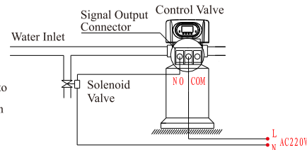
Figure 3-3 Wiring of Pressure Relief
