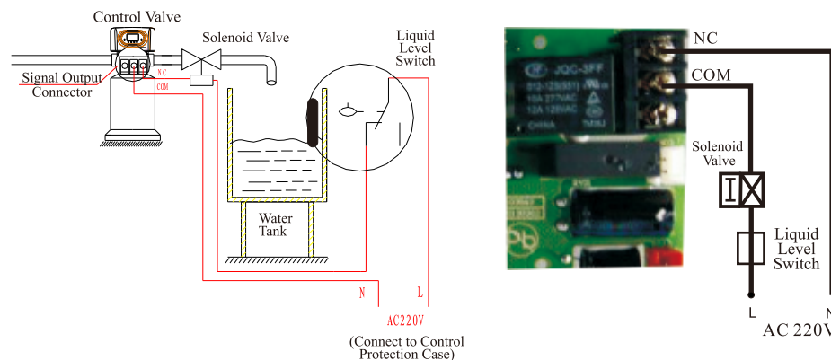
Figure 3-1 Wiring of Solenoid Valve on Outlet
