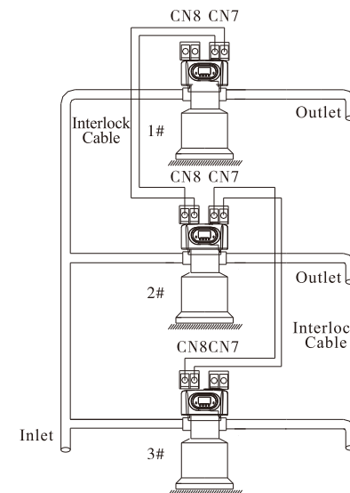
Figure 3-10 Interlock system
