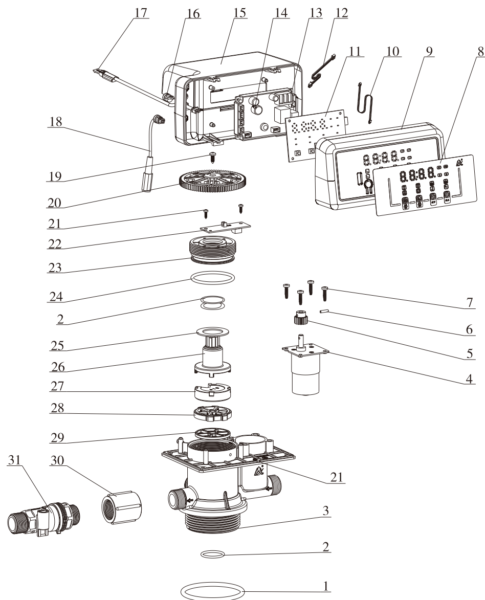
F71S3爆炸图
